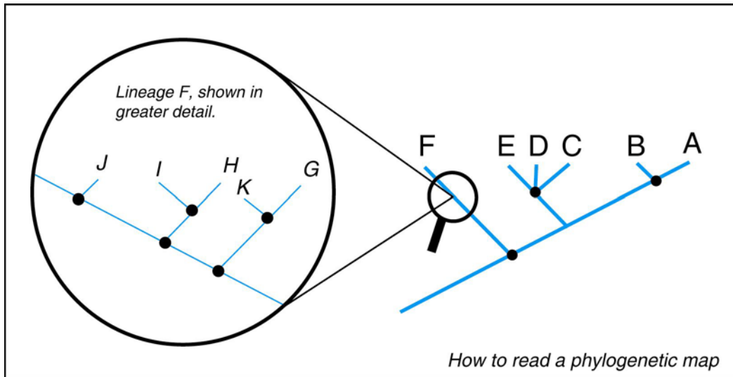
Fig. 11.05 Like geographic maps of different scales, branches on a phylogenetic map, like those labeled A - F, may consist of a single species, or thousands of related species. Branch F, for example, might represent hundreds of species that are simply depicted as a single lineage.
