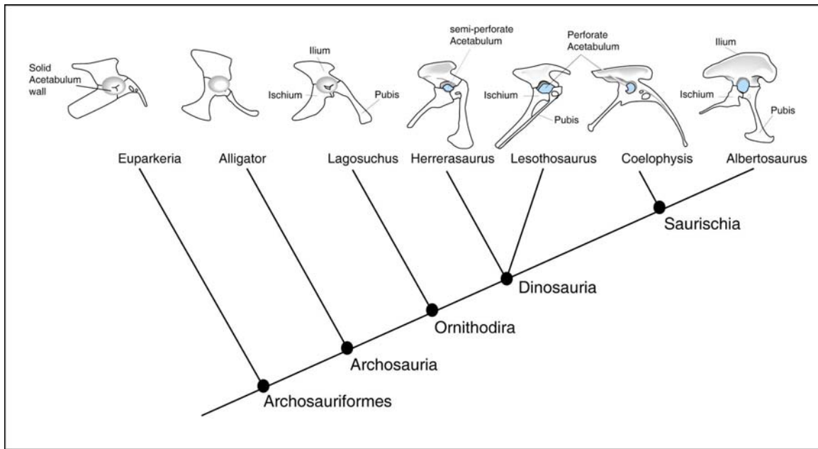
Figure 11.28 These archosaur pelvises show the primitive closed socket acetabulum, compared with the perforated acetabulum (blue) of dinosaurs.
