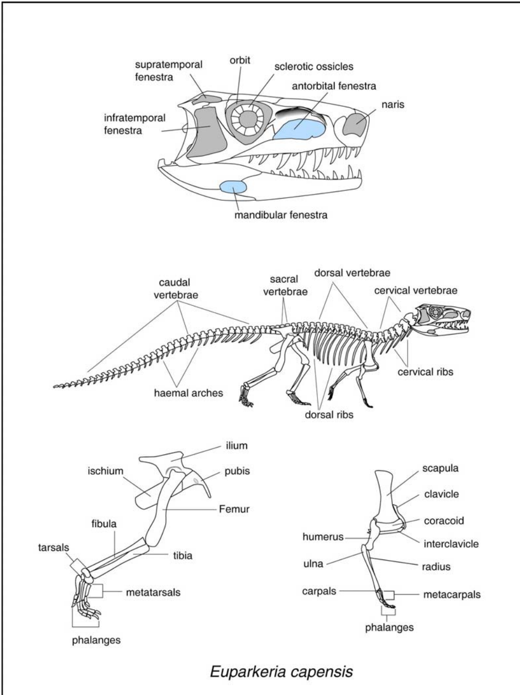
Fig. 11.21 Basic archosaur skeletal anatomy, illustrated by Euparkeria.
