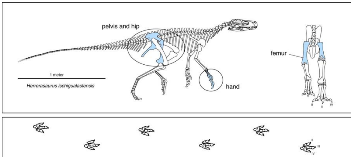
Fig. 11.24 Diagnostic regions of the dinosaur skeleton are the pelvis, hip, and hand, illustrated here by Herrerasaurus . The hip modifications locked dinosaurs into a narrow gait. The hands could grasp, much as our own hands can.
